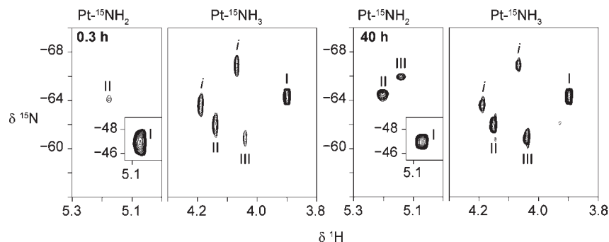
Figure 2. Two-dimensional [ ^1\text{H} , ^{15}\text{N} ] HSQC NMR spectra of ^{15}\text{N} -labeled 1 in 15 mM sulfate (95% \text{H}_2\text{O}/5\% \text{D}_2\text{O} ) at pH 5.4 and 298 K at the start of the reaction (0.3 h) and at equilibrium (40.3 h). The resonances are assigned to the \text{Pt}-^{15}\text{NH}_2 and \text{Pt}-^{15}\text{NH}_3 groups of the \text{Pt}-\text{Cl} (I), \text{Pt}-\text{OH}_2 (II), and \text{Pt}-\text{SO}_4 (III) species and correspond to the mononuclear derivative of 1,1/t,t , [\text{trans-Pt}(\text{NH}_3)_2(\text{NH}_2(\text{CH}_2)_6\text{NH}_2)\text{Y}]^{n+} , where Y represents any other ligand (see Scheme 1). Peak assignments are shown in Table 1. Peaks labeled 'i' are assigned to ^{15}\text{N} impurities from the synthesis of ^{15}\text{N} - 1 ; their presence does not compromise these experiments, as discussed in detail elsewhere. 23
